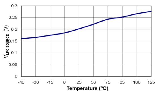
Figure 13. LPC Lower Clamp Voltage
