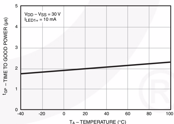
Figure 28. Time to Good Power ( t_{GP} ) vs. Temperature
