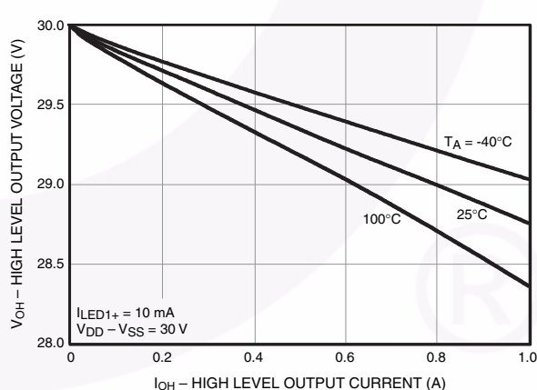
Figure 10. High Level Output Voltage ( V_{OH} ) vs. High Level Output Current ( I_{OH} )
