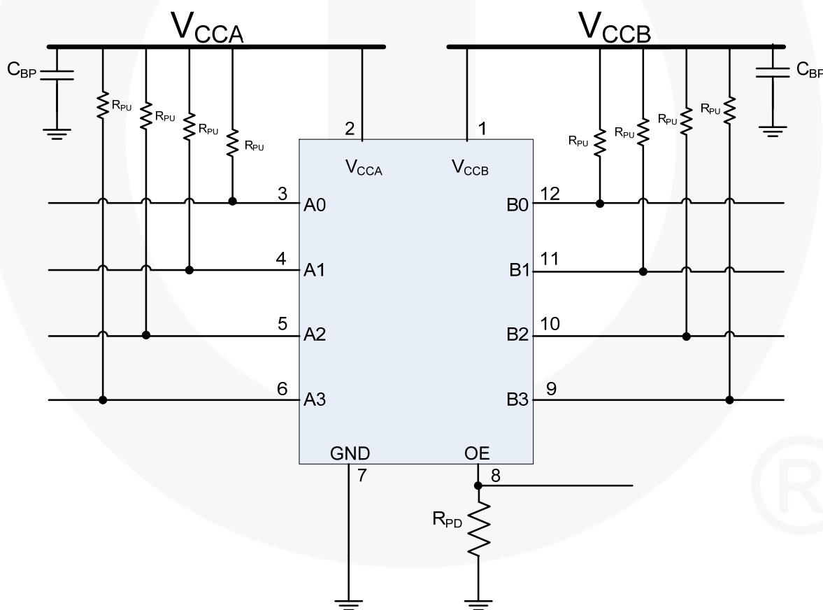
Figure 3. Application Circuit
