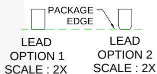
Figure 15. 12-Lead Ultrathin MLP, 1.8mm x 1.8mm
