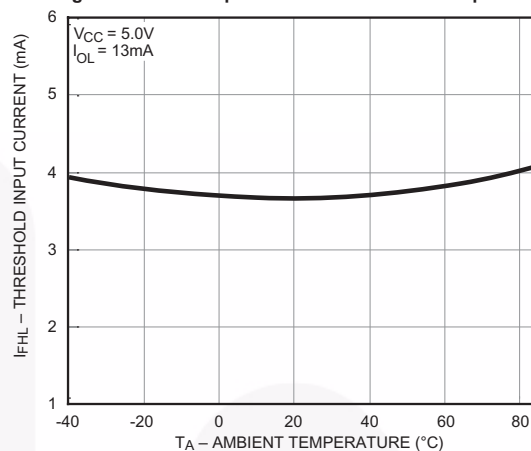
Fig. 2 Threshold Input Current vs Ambient Temperature
