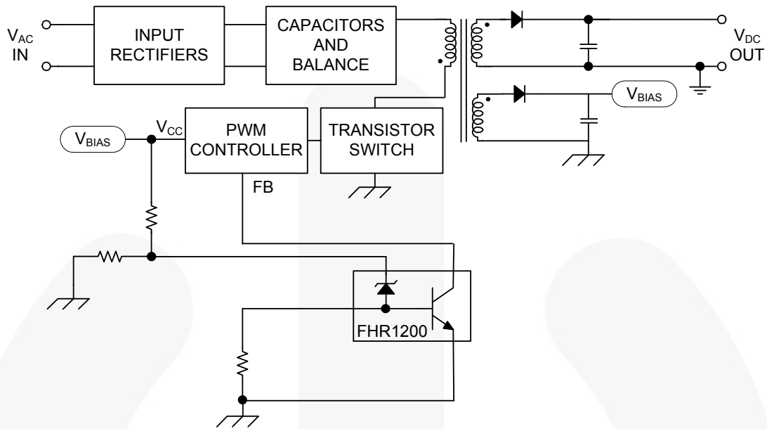
Figure 21. Flyback Power Supply Primary-Side Regulation
